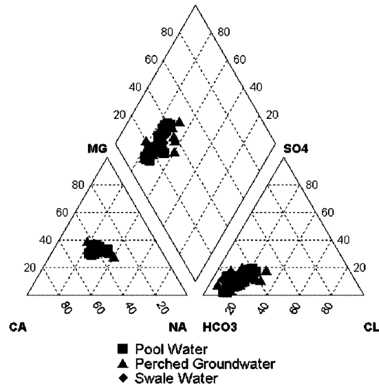
Figure 6. Piper diagrams summarizing the relative concentrations of the major cations and anions in vernal pool water (squares), perched groundwater (triangles), and outlet swale water just upgradient of the seasonal stream (diamonds). All surface water and perched groundwater samples are included. All surface water and perched groundwater samples plot as Ca–Mg–Na–HCO 3 , which is typical of regional rainfall that has undergone slight alteration due to short-term contact with sediments
